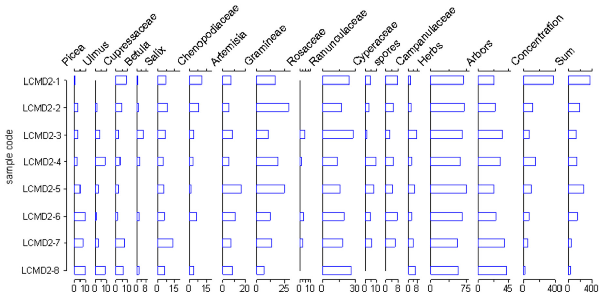
Fig. 4. Pollen percentages in bulk samples from the second layer of Longquan Cave deposits.
