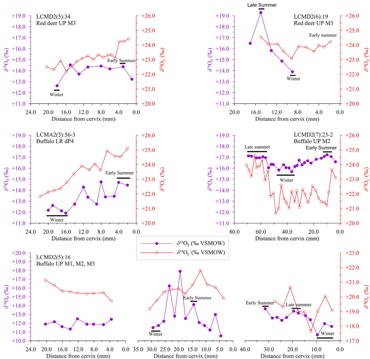
Fig. 3. Intra-tooth variations in oxygen isotope compositions of bioapatite phosphate ( \delta^{18}\text{O}_p in ‰, VSMOW), compared to data for bioapatite structural carbonate ( \delta^{18}\text{O}_c in ‰, VSMOW) in tooth enamel of seven fossil teeth. The \delta^{18}\text{O}_p and \delta^{18}\text{O}_c show generally similar changing patterns in the same tooth. Seasons were assigned according to the peaks and troughs of \delta^{18}\text{O}_p and \delta^{18}\text{O}_c curves, as shown by horizontal bars.
