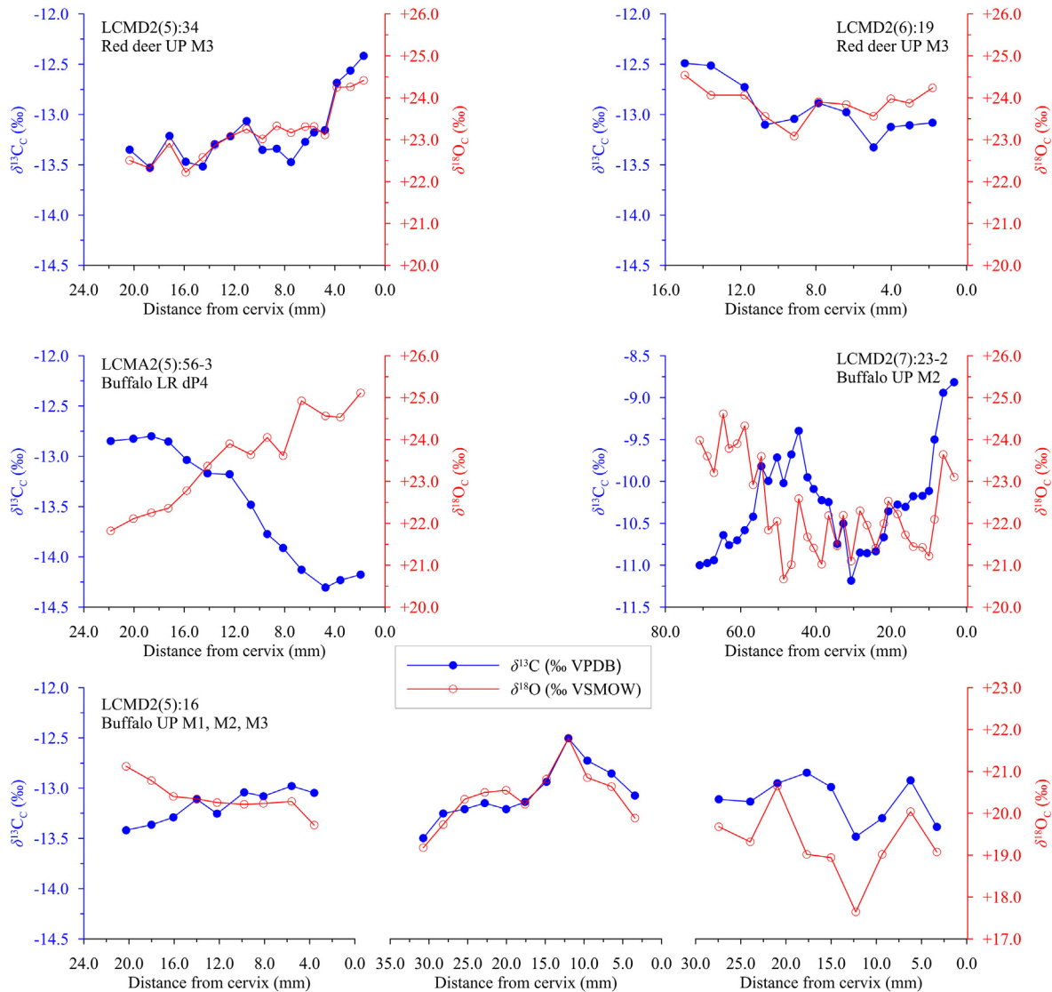
Fig. 2. Intra-tooth variations in stable carbon and oxygen isotope compositions of bioapatite structural carbonate ( \delta^{13}\text{C} in ‰, VPDB; \delta^{18}\text{O} in ‰, VSMOW) in tooth enamel of seven fossil teeth versus distance (in mm) from the cervix.
