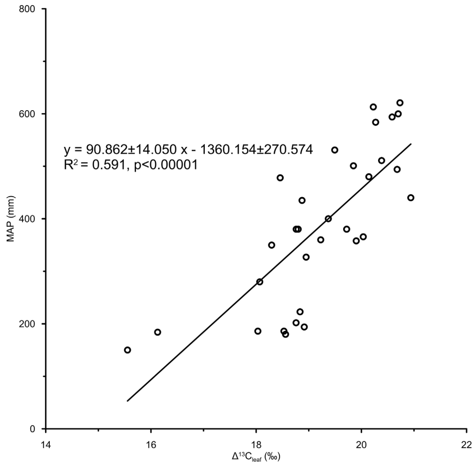
Fig. 5. Correlation between Mean Annual Precipitation (MAP) (mm) and the carbon isotope fractionation (‰) between modern C_3 plants and atmospheric carbon dioxide ( \Delta_{\text{leaf-atm CO}_2} ). Data are from Wang et al. (2003).
